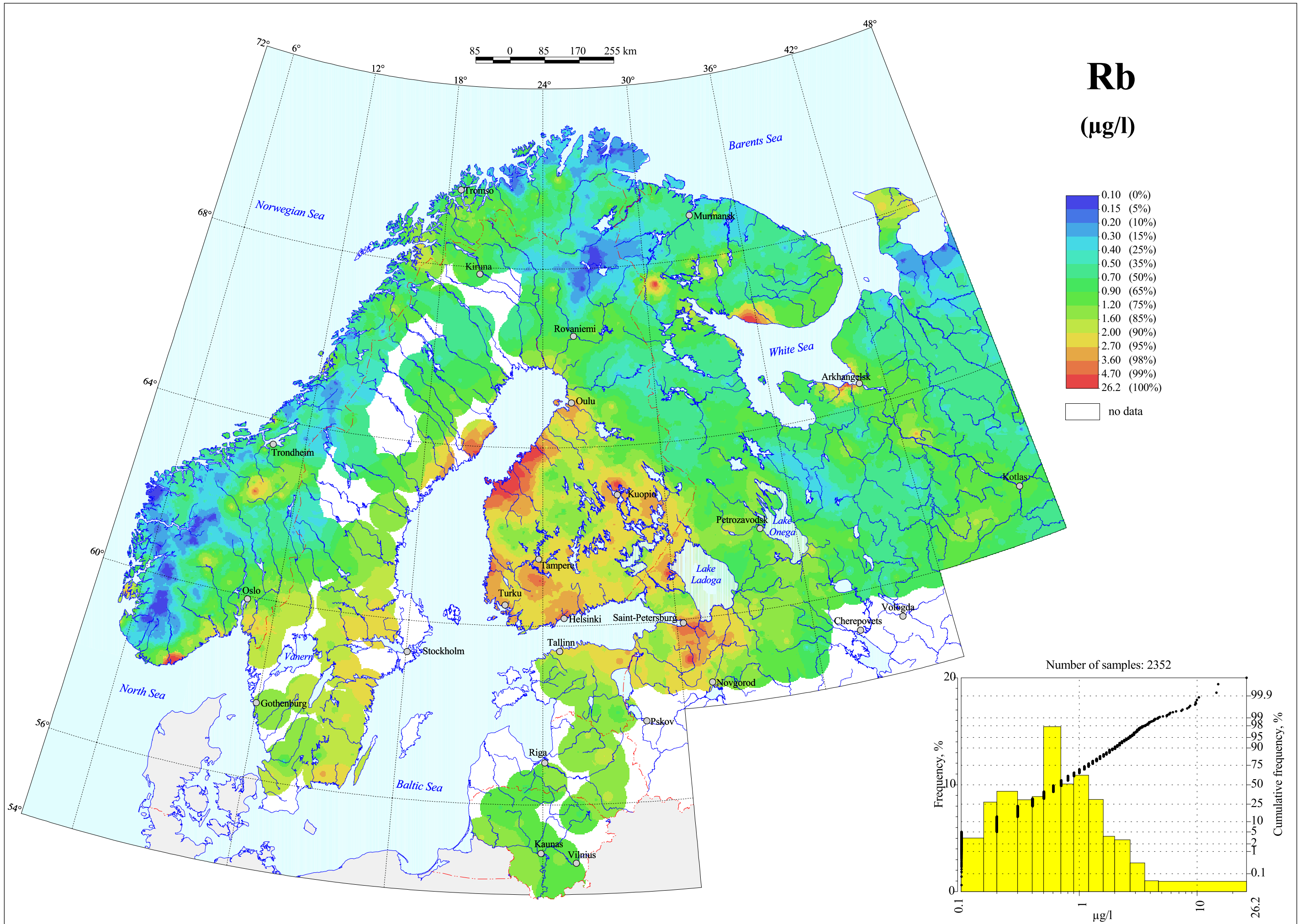
Rubidium in Surface Water
